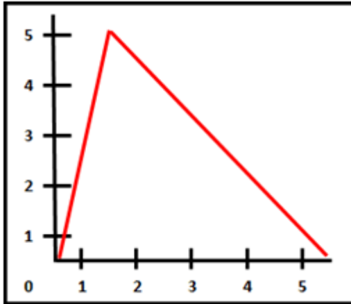
Triangular Distribution Curves
