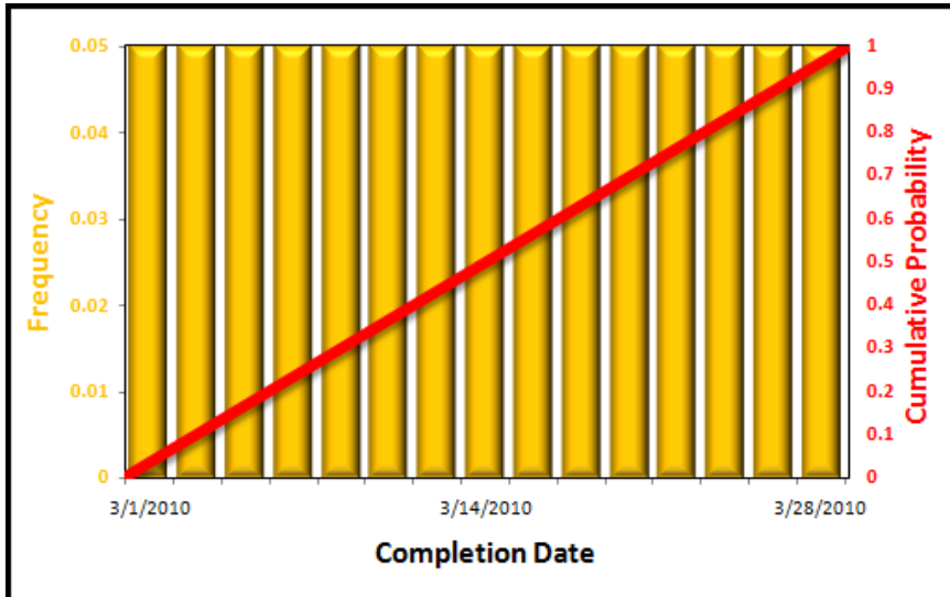
Uniform Distribution Curve
