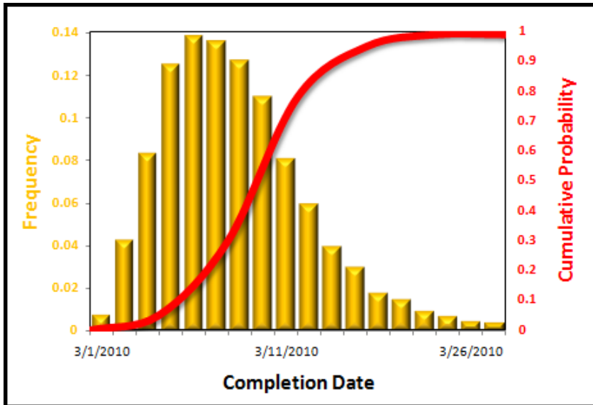
Beta Distribution Curve (2)
